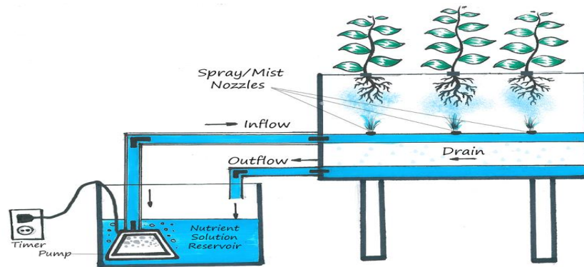
Fig. 1. Working of aeroponics system
