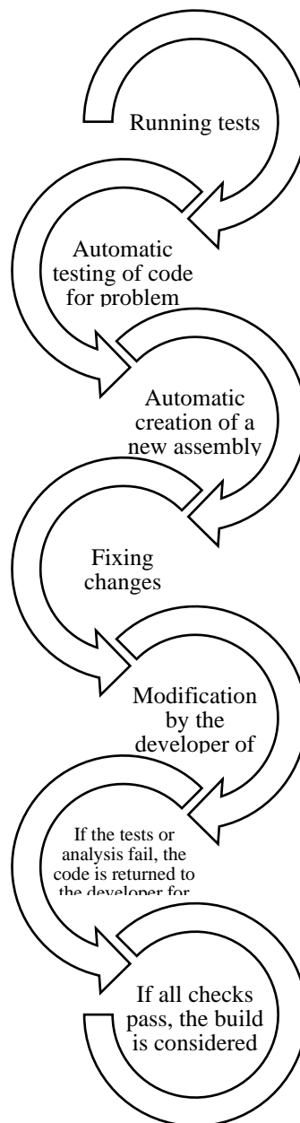
Fig. 1. Approximate operation of the CI/CD pipeline (CI/CD, 2024)
